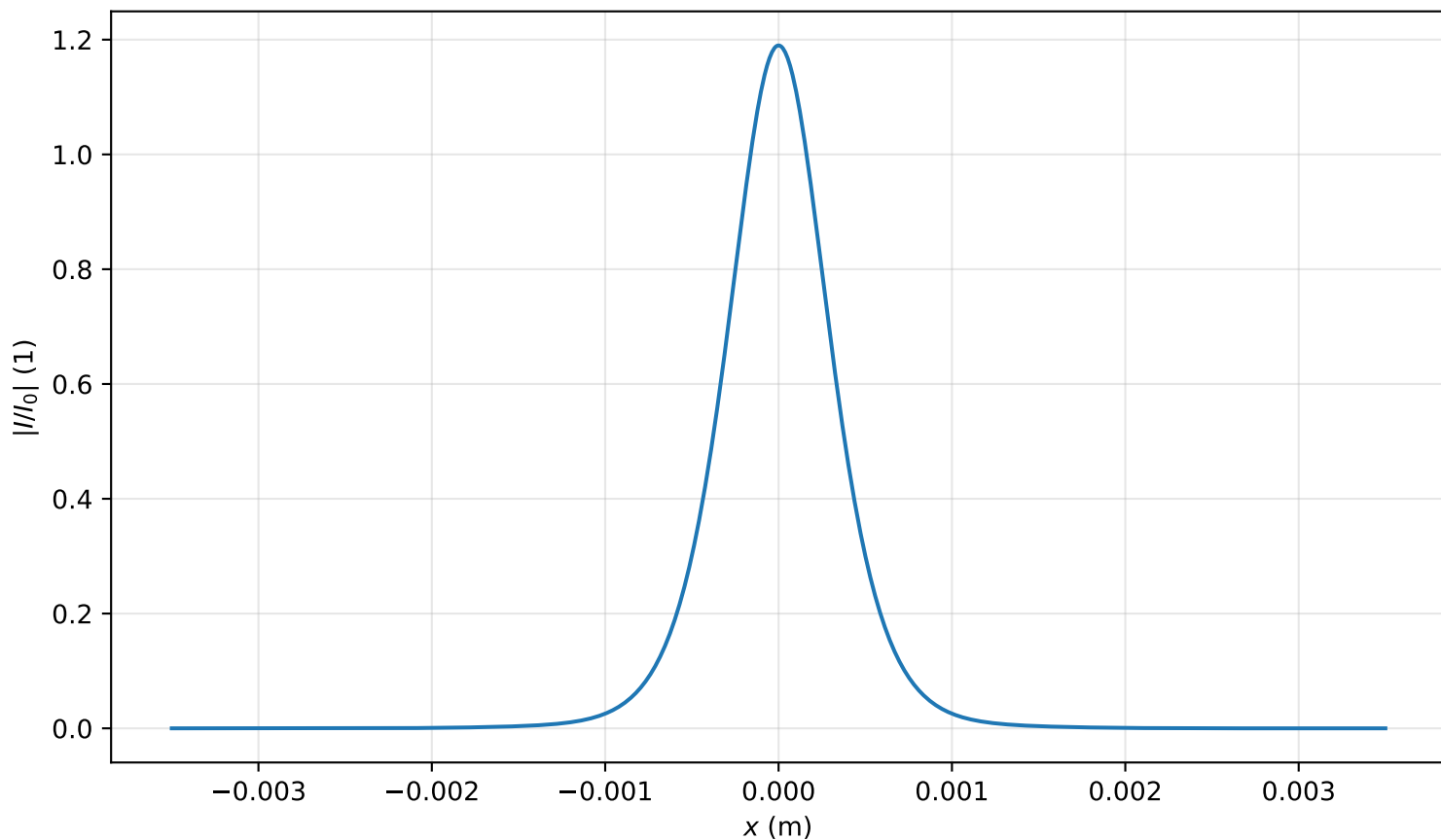
Intensity profile I(x, y = 0, z = 2.627m)/I_0 , P_{in}=0.8P_{cr} , artificial time
